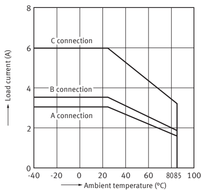
1-4. Load current vs. ambient temperature characteristics
