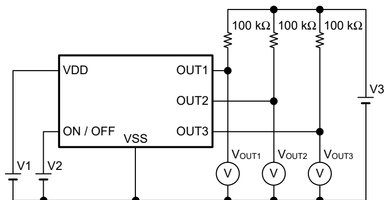
Figure 4 Test Circuit 1
