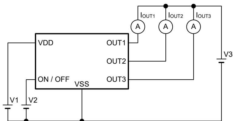
Figure 6 Test Circuit 3
