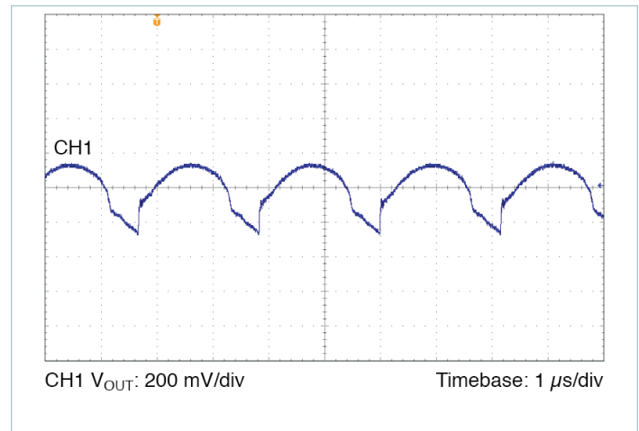
Figure 18 — Output voltage ripple, V_{IN} = 28\text{V} , V_{OUT} = 5.0\text{V} , C_{OUT\_EXT} = 1000\mu\text{F} , R_{LOAD} = 0.139\Omega
