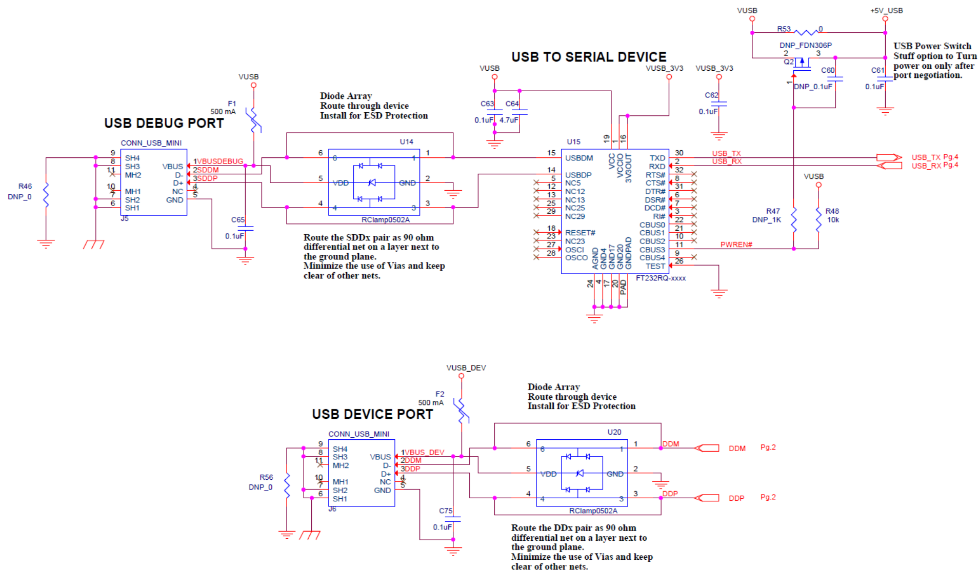
Figure 2-15 Evaluation Board Schematic for XPCW1003100K, Part 7 of 7
