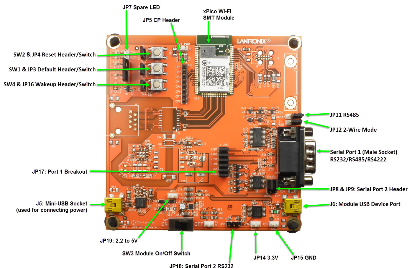
Figure 2-2 xPico Wi-Fi SMT Evaluation Board XPW100300K – Connectors and Jumpers
