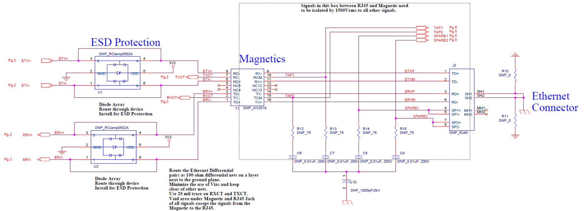
Figure 2-14 Evaluation Board Schematic for XPCW1003100K, Part 6 of 7
