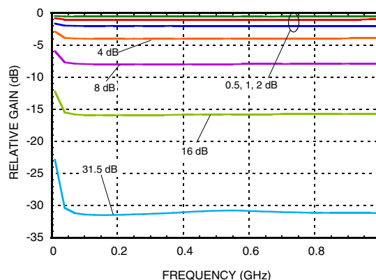
Output Attenuator Relative Attenuation [4] (Major States)
