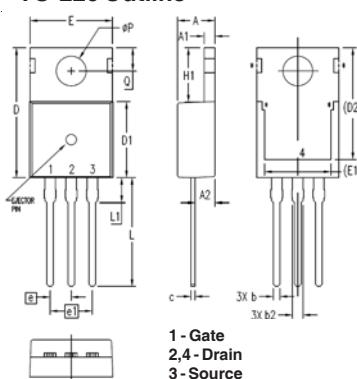
TO-220 Outline
