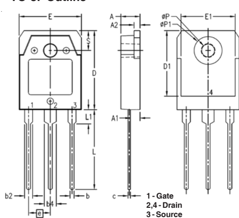
TO-3P Outline
