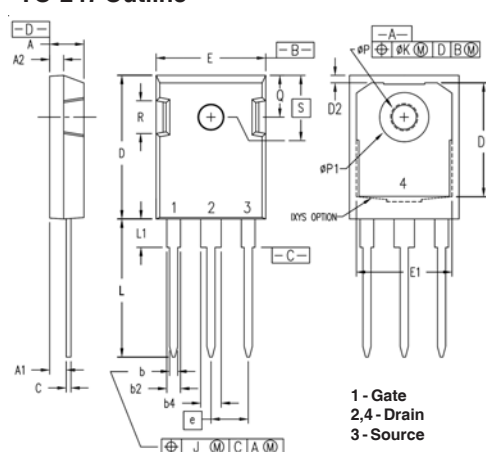
TO-247 Outline
