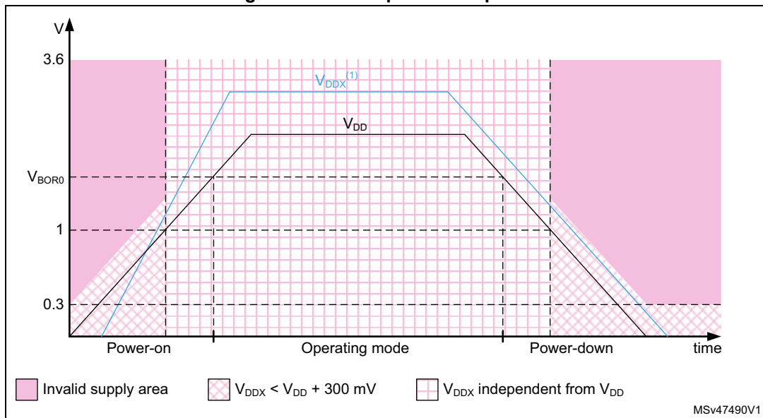
Figure 5. Power-up/down sequence
