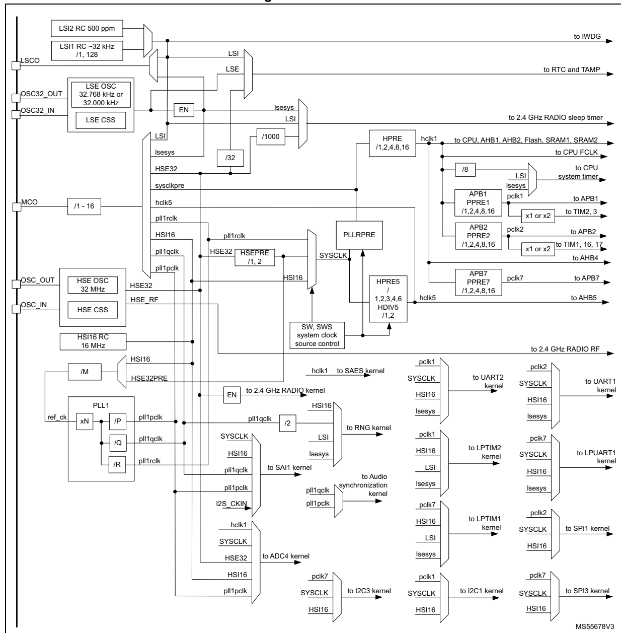
Figure 6. Clock tree
