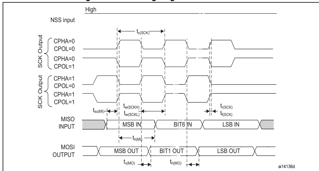
Figure 31. SPI timing diagram - Master mode
