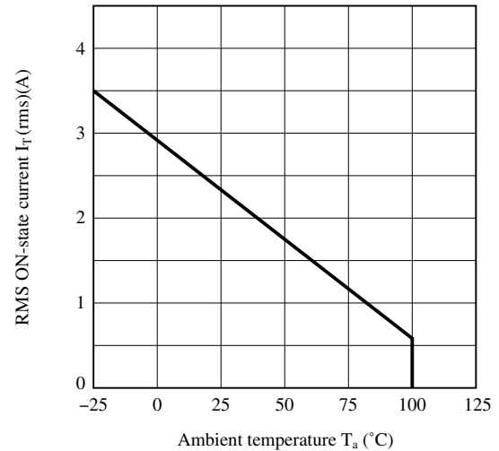
Fig.2 RMS ON-state Current vs. Ambient Temperature
