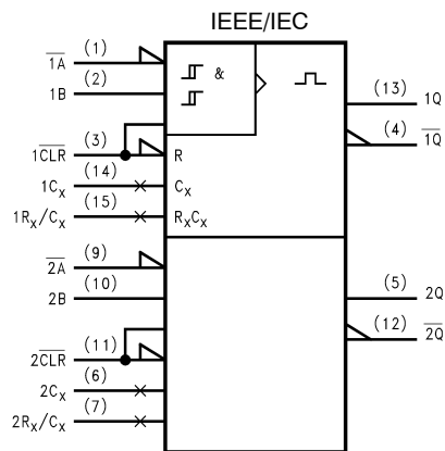
Figure 2. Logic Symbol
