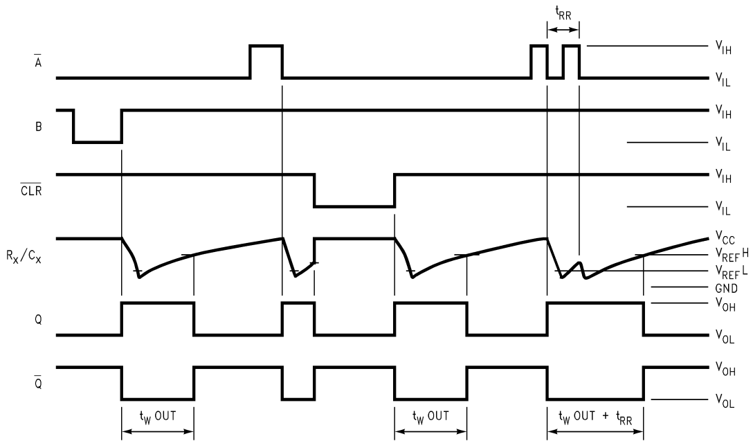
Figure 5. Timing Chart
