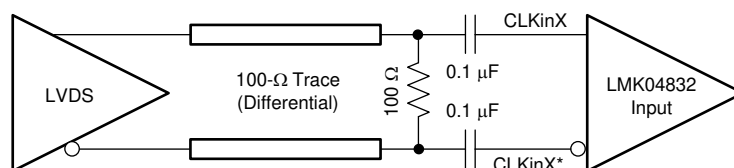
Figure 9-1. CLKInX/X* or OSCIn Termination for an LVDS Reference Clock Source
