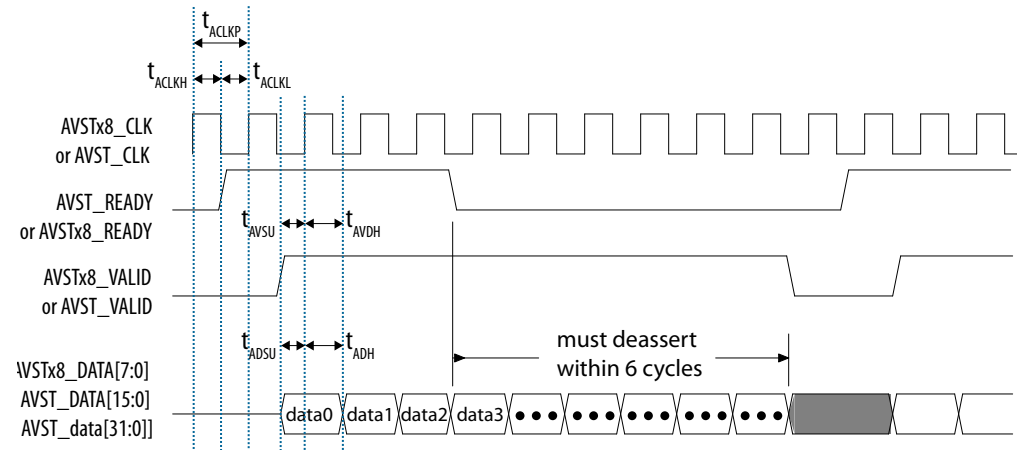
Figure 30. Avalon-ST Configuration Timing Diagram
