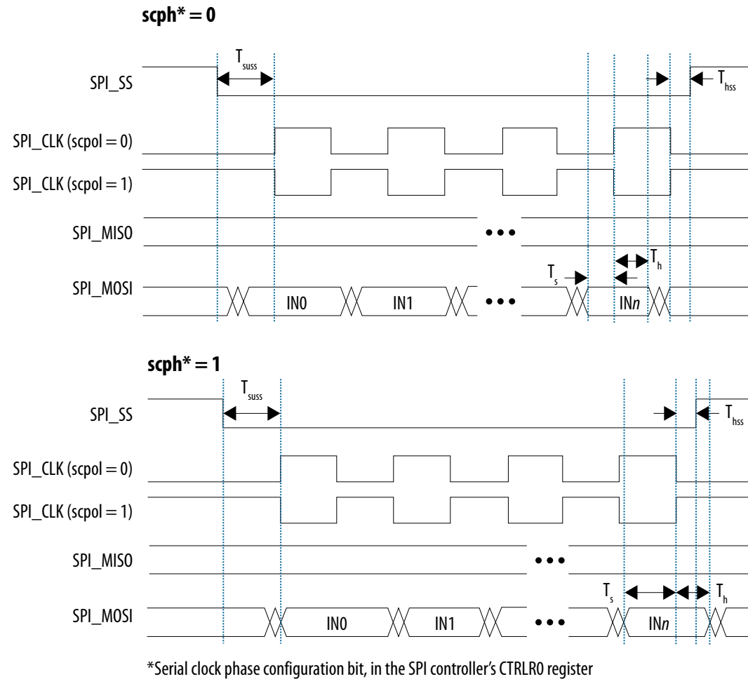
Figure 8. SPI Slave Input Timing Diagram
