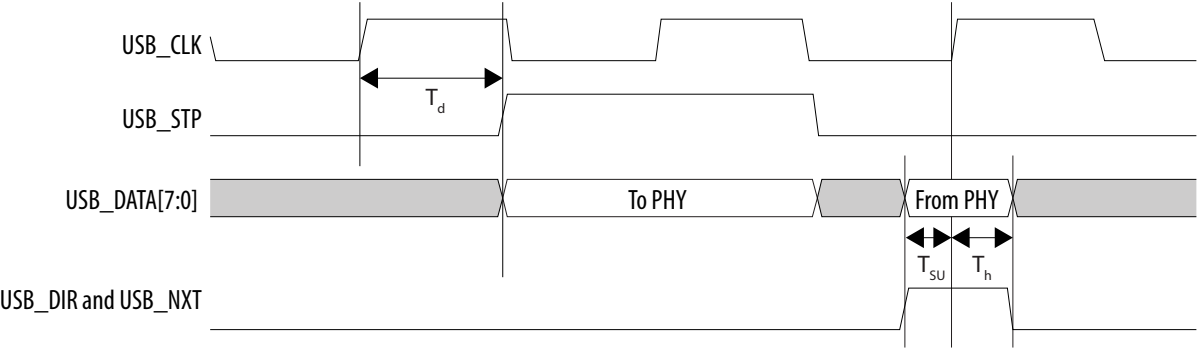
Figure 10. USB ULPI Timing Diagram
