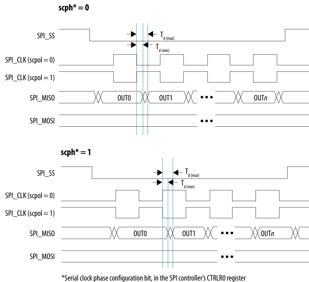
Figure 7. SPI Slave Output Timing Diagram
