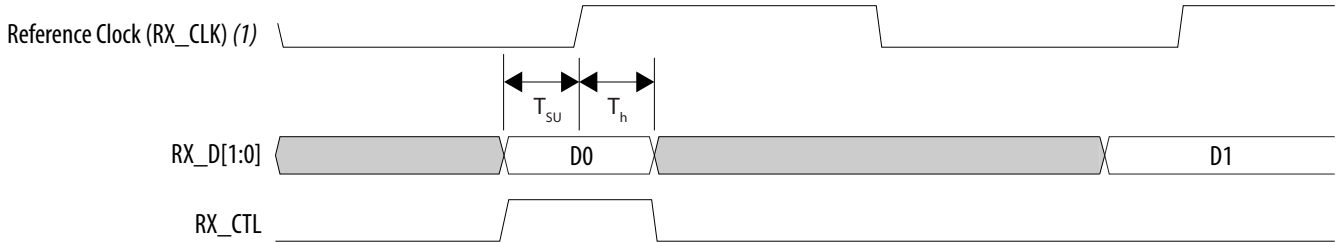
Figure 14. RMII RX Timing Diagram
