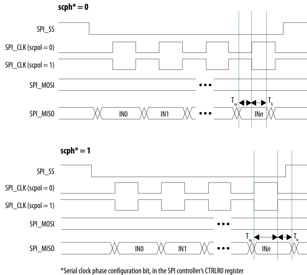
Figure 6. SPI Master Input Timing Diagram
