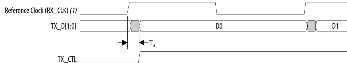
Figure 13. RMII TX Timing Diagram
