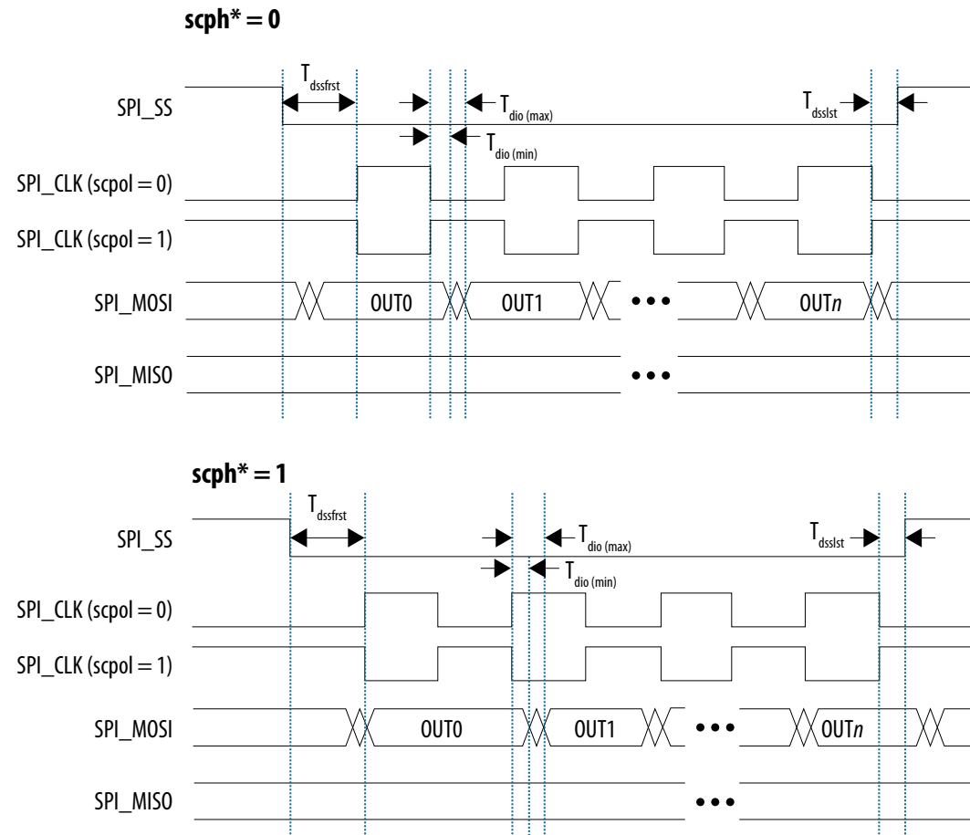
Figure 5. SPI Master Output Timing Diagram
