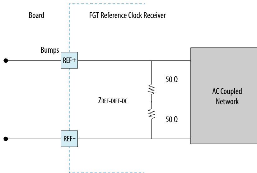
Figure 4. Simplified F-Tile FGT Reference Clock Input Buffer
