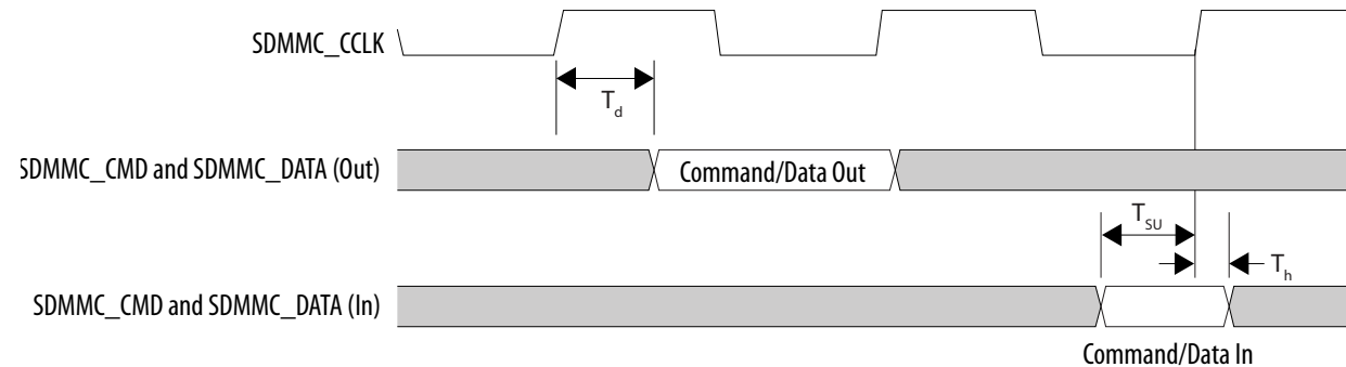
Figure 9. SD/MMC Timing Diagram
