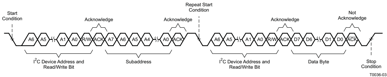
Figure 52. Read Transfer
