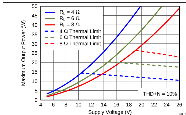
Figure 1. Output Power vs PVDD
