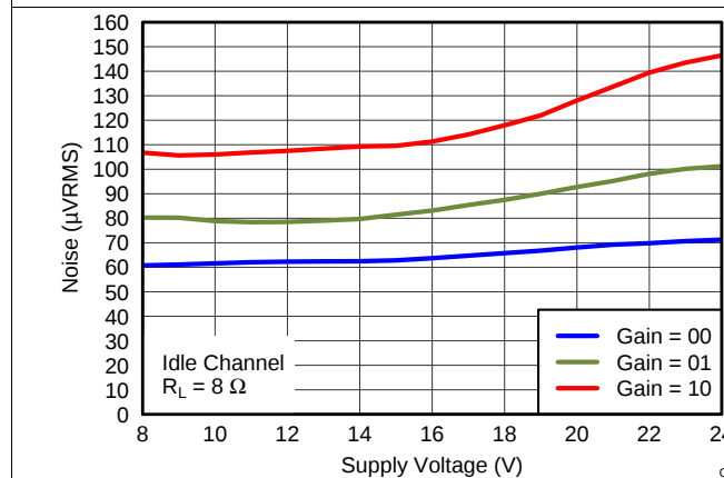
Figure 30. Idle Channel Noise vs PVDD
