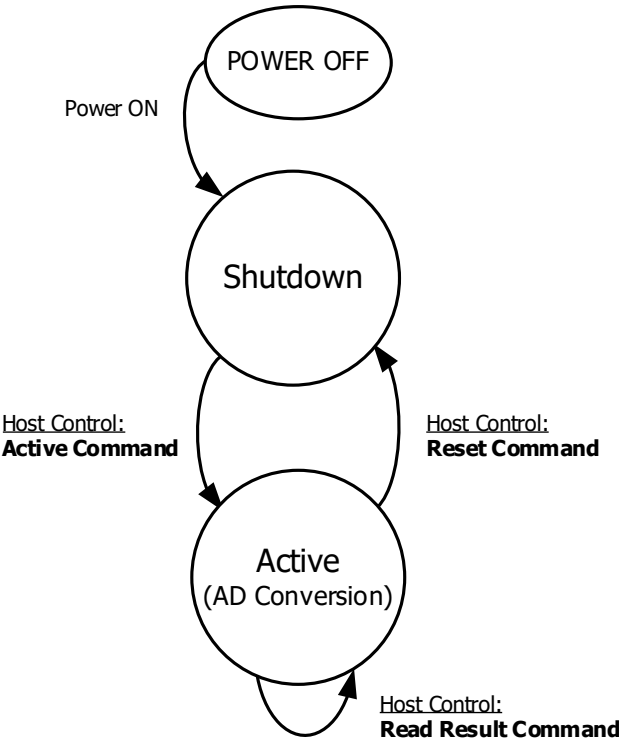
Fig. 10 State transition diagram
