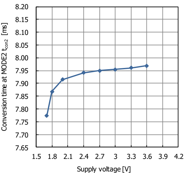
Fig.13.12 Conversion time at MODE2 t_{con2} supply voltage characteristic
