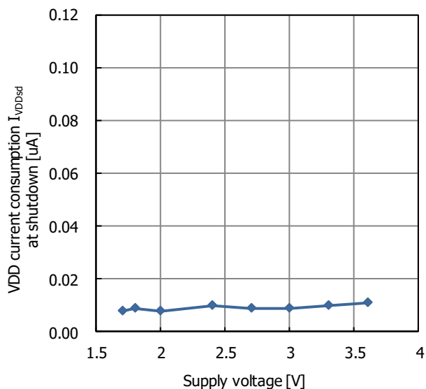
Fig.13.4 VDD current consumption I_{VDDsd} at shutdown supply voltage characteristic
