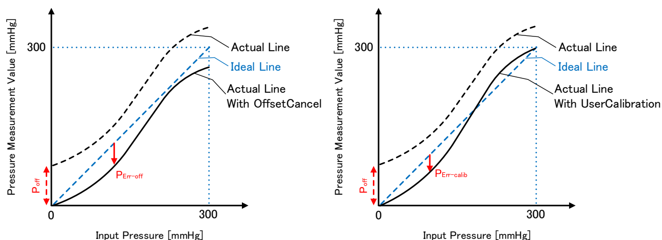
Fig. 4 Definition of Characteristics
