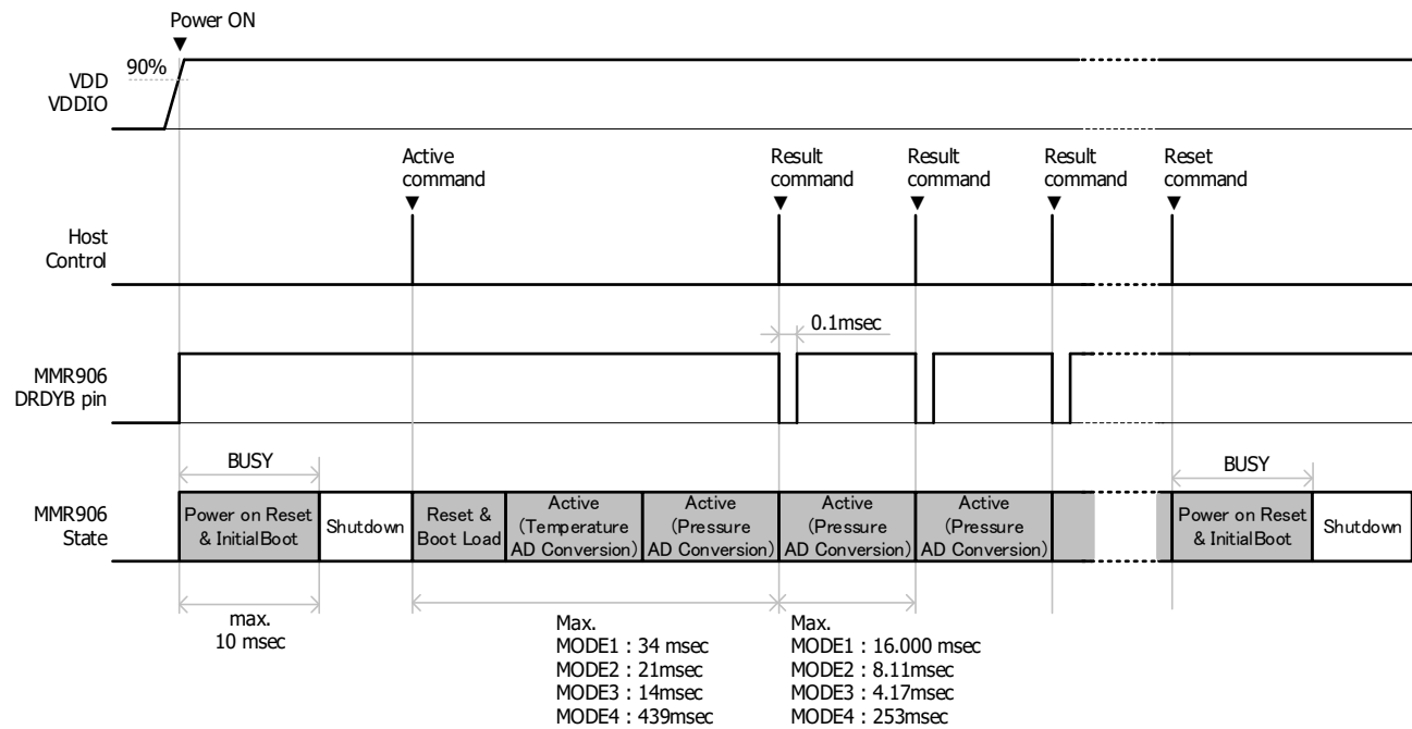
Fig. 11 Timing Chart
