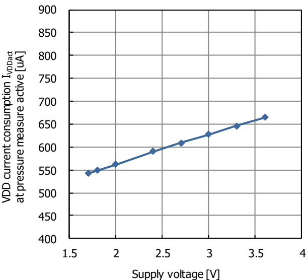
Fig.13.2 VDD current consumption I_{VDDact} at pressure measure active supply voltage characteristic
