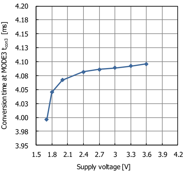
Fig.13.14 Conversion time at MODE 3 supply voltage characteristic
