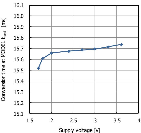
Fig.13.10 Conversion time at MODE1 t_{con1} supply voltage characteristic
