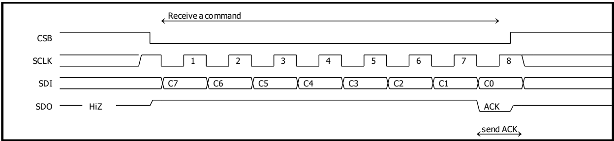
Fig. 7 SPI Operation Command format
