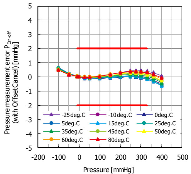
Fig.13.19 Pressure measurement error P_{Err-Off} (with Offset Cancel) temperature characteristic
