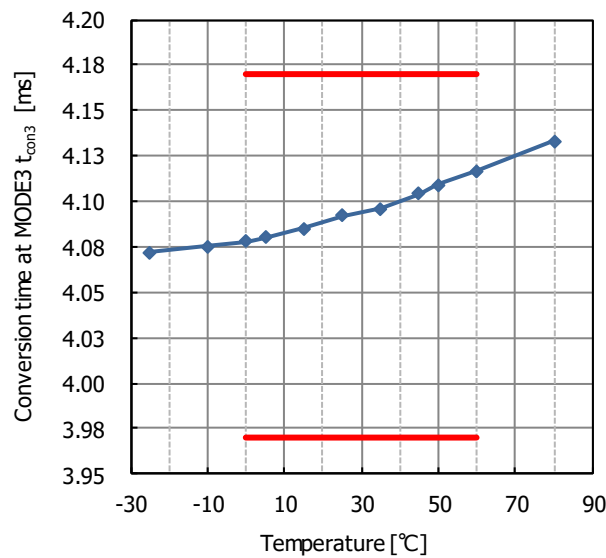
Fig.13.13 Conversion time at MODE 3 temperature characteristic
