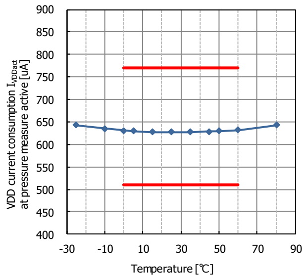
Fig. 13.1 VDD current consumption I_{VDDact} at pressure measure active temperature characteristic
