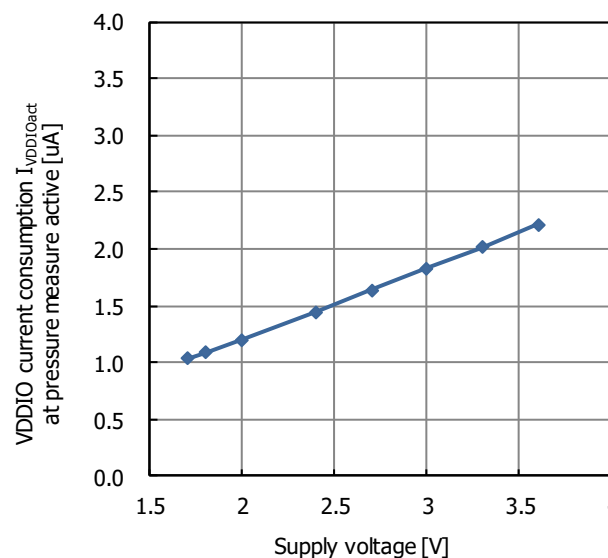
Fig.13.6 VDDIO current consumption I_{VDDIOact} at pressure measure active supply voltage characteristic
