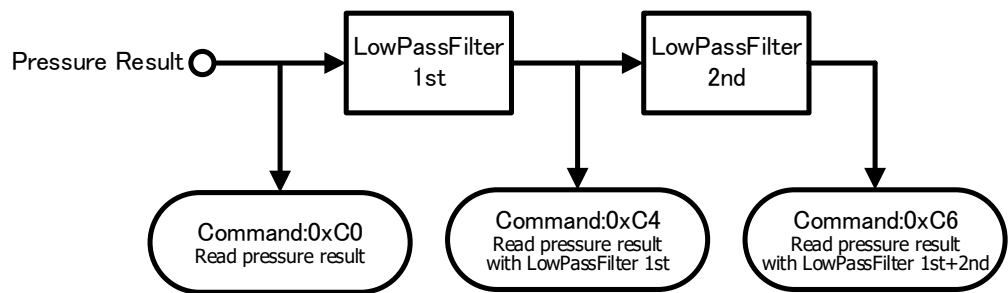
Fig. 5 LowPassFilter Configuration
