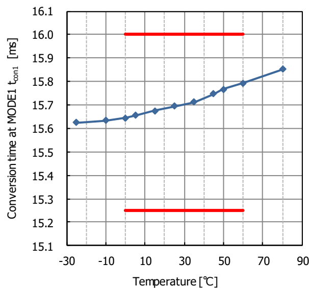
Fig.13.9 Conversion time at MODE1 t_{con1} temperature characteristic
