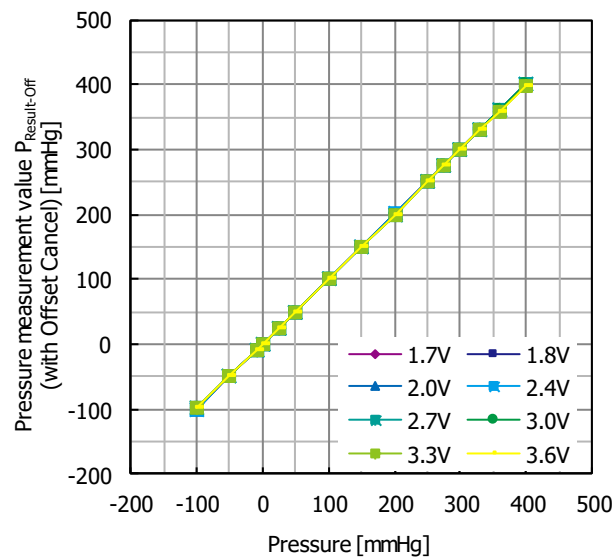
Fig.13.18 Pressure measurement value P_{Result-Off} (with Offset Cancel) supply voltage characteristic
