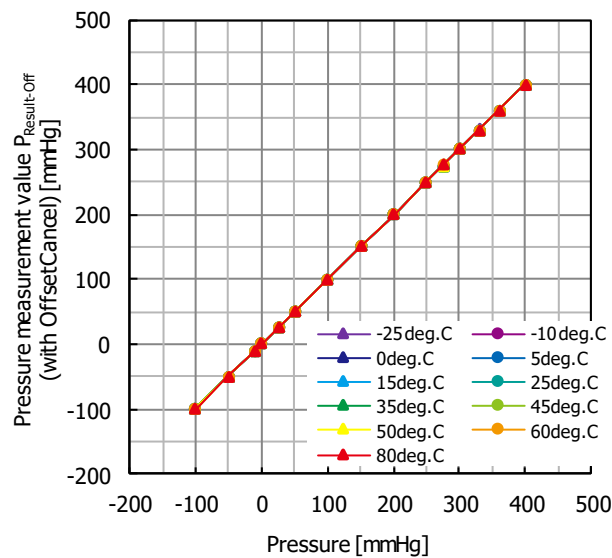
Fig.13.17 Pressure measurement value P_{Result-Off} (with Offset Cancel) temperature characteristic
