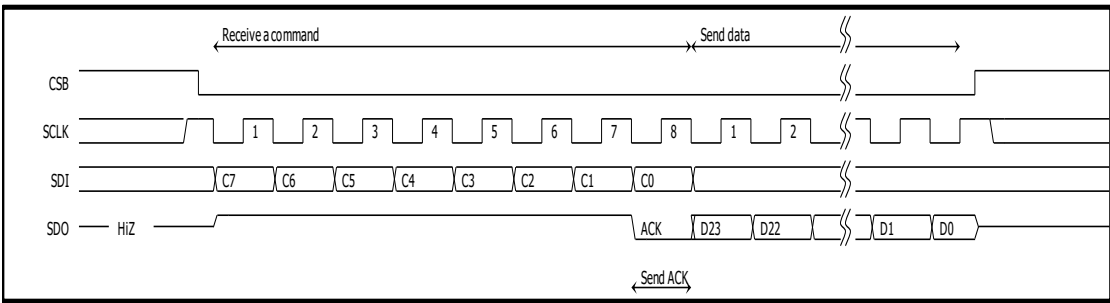
Fig. 8 SPI Result Command format
