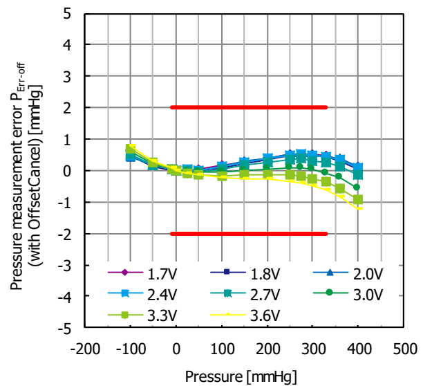
Fig.13.20 Pressure measurement error P_{Err-Off} (with Offset Cancel) supply voltage characteristic
