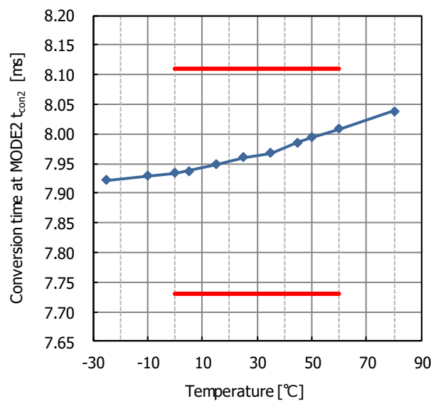
Fig.13.11 Conversion time at MODE2 t_{con2} temperature characteristic
