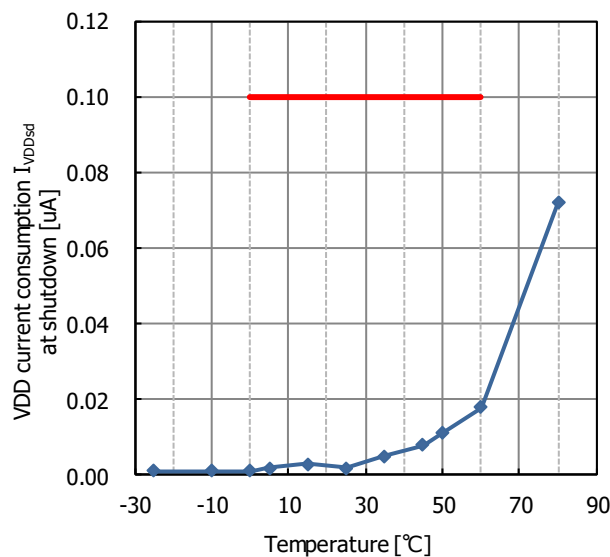
Fig.13.3 VDD current consumption I_{VDDsd} at shutdown temperature characteristic
