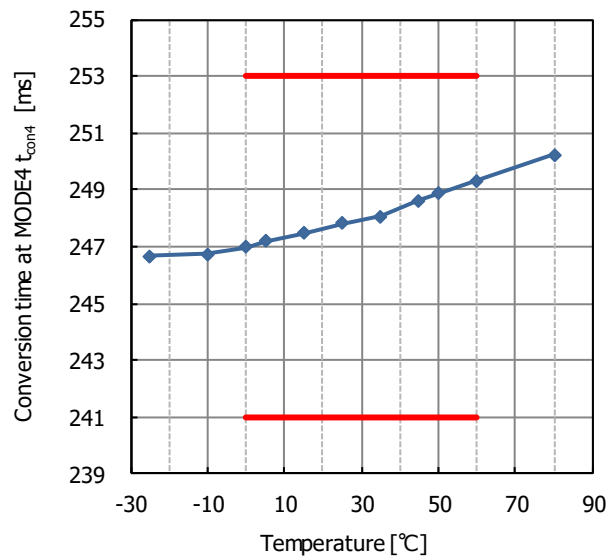
Fig.13.15 Conversion time at MODE 4 temperature characteristic
