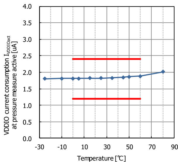
Fig.13.5 VDDIO current consumption I_{VDDIOact} at pressure measure active temperature characteristic
