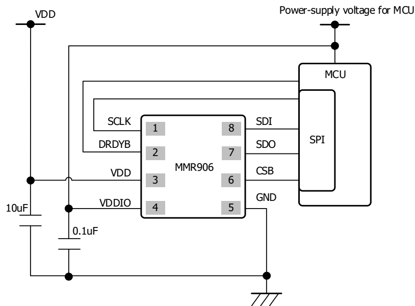
Fig. 12 Typical Electrical Connection
