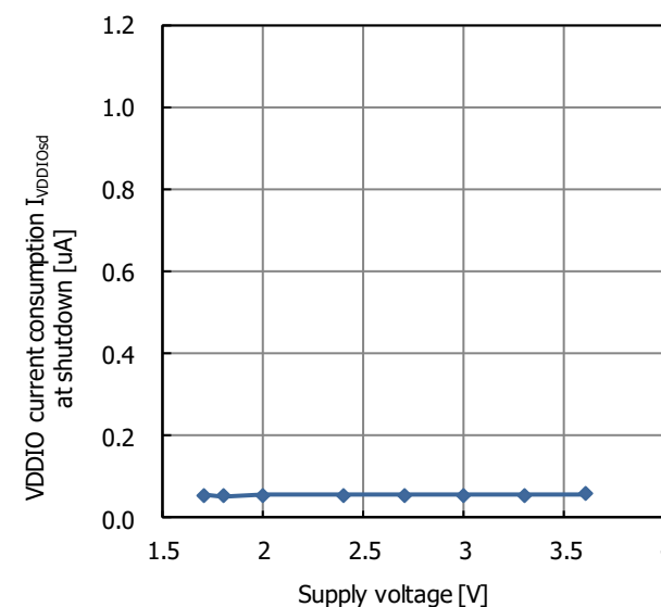
Fig.13.8 VDDIO current consumption I_{VDDIOsd} at shutdown supply voltage characteristic
