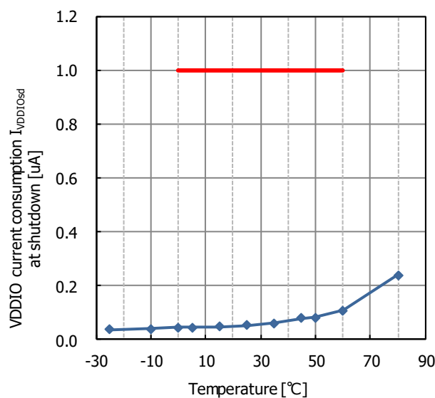
Fig.13.7 VDDIO current consumption I_{VDDIOsd} at shutdown temperature characteristic
