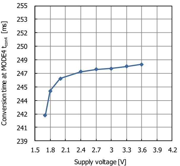
Fig.13.16 Conversion time at MODE 4 supply voltage characteristic
