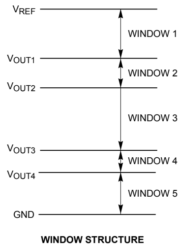
WINDOW STRUCTURE
