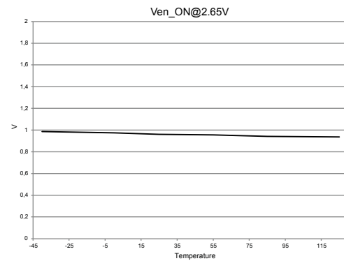
Figure 20. Enable threshold vs. temperature
