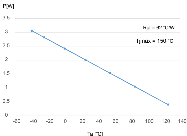
Figure 6. Derating curve
