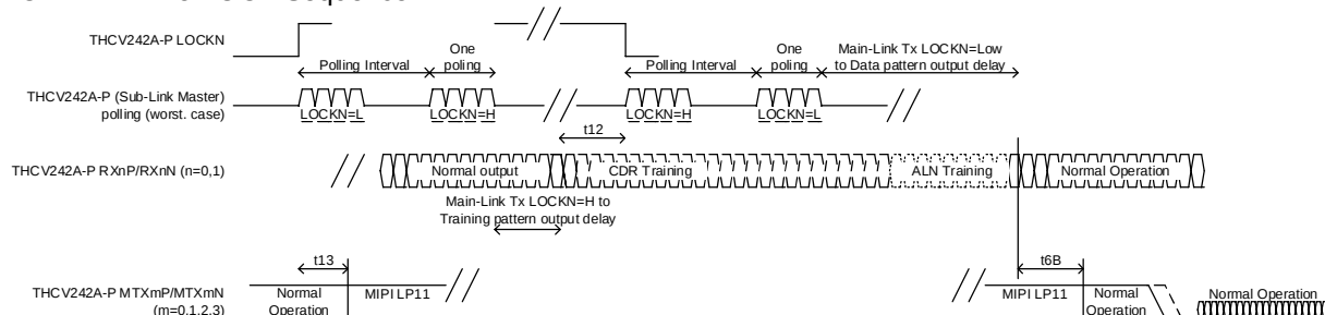
Figure 18. Re-Lock Sequence
