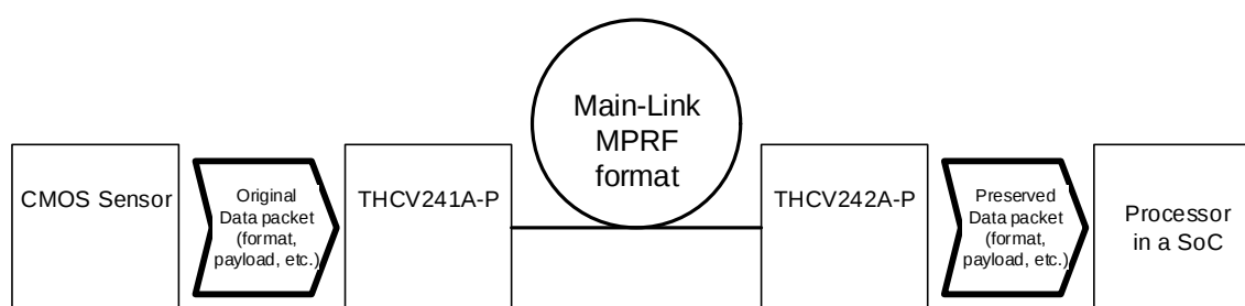
Figure 2. MPRF (Main-Link PRivate Format)
