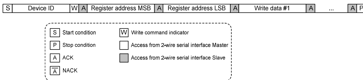
Figure 5. 2-wire serial I/F write to THCV242A-P local register protocol
