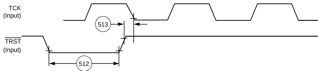
Figure 2-49. \overline{\text{TRST}} Timing Diagram
