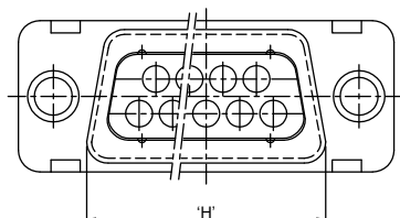
STD-THROUGH HOLE.
