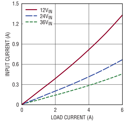
LTM8053 Input vs Load Current V_{OUT} = 2\text{V} , BIAS = 5V
