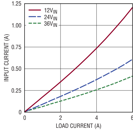
LTM8053 Input vs Load Current V_{OUT} = 1.8\text{V} , BIAS = 5V
