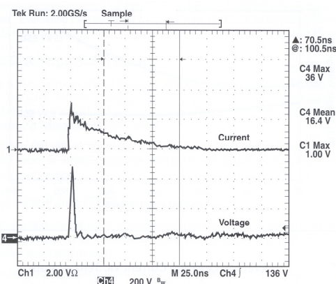
Figure 1. Typical Device Characteristics
