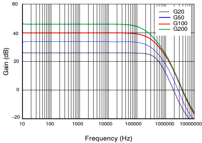
Figure 12. Gain vs Frequency
