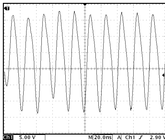
Fig. 17 50MHz Burst Repetition Frequency
