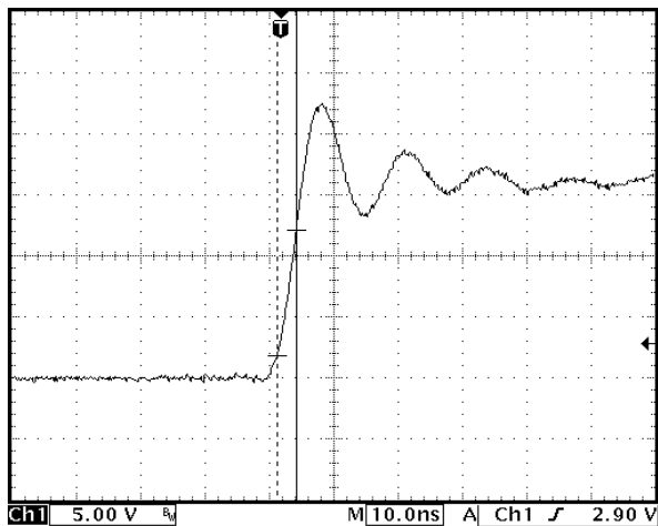
Fig. 14 <8ns Minimum Pulse Width
