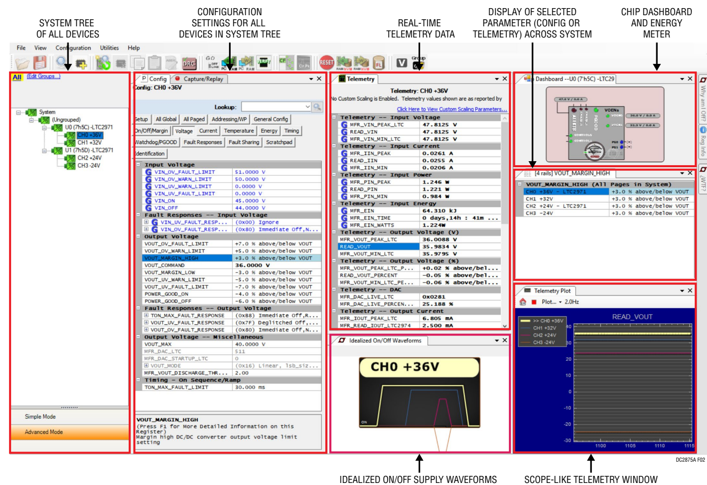
Figure 2. Screenshot of the LTpowerPlay GUI
