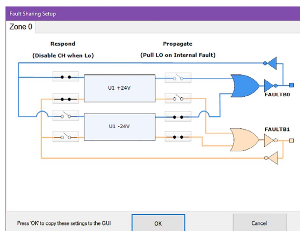
Figure 10. Updated Fault Sharing Configuration
