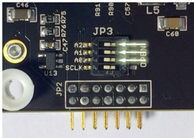
Figure 15. DIP Switch Set to All 0's
