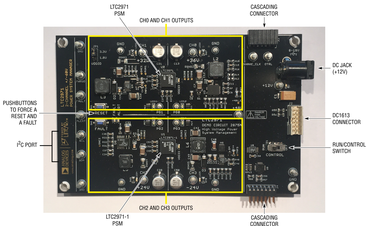
Figure 4. DC2875A Details
