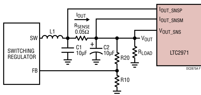
Figure 11. Switcher with Sense Resistor
