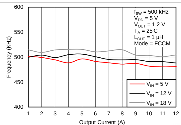
Figure 56. Switching Frequency vs. Output Current
