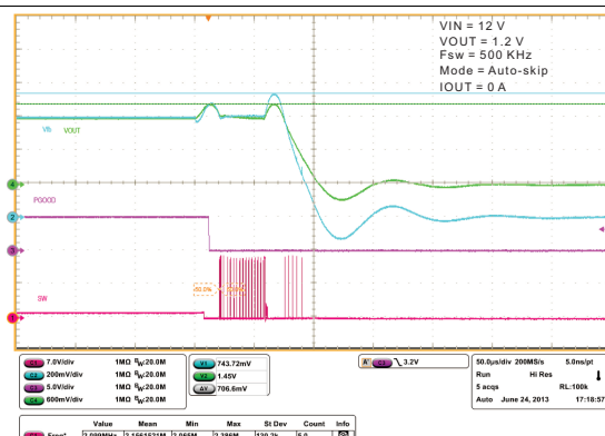
Figure 30. Overvoltage Protection
