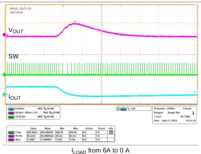
Figure 60. Load Transient
