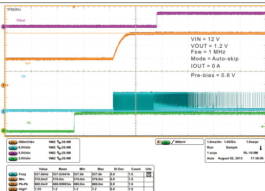
Figure 29. Pre-Bias Operation
