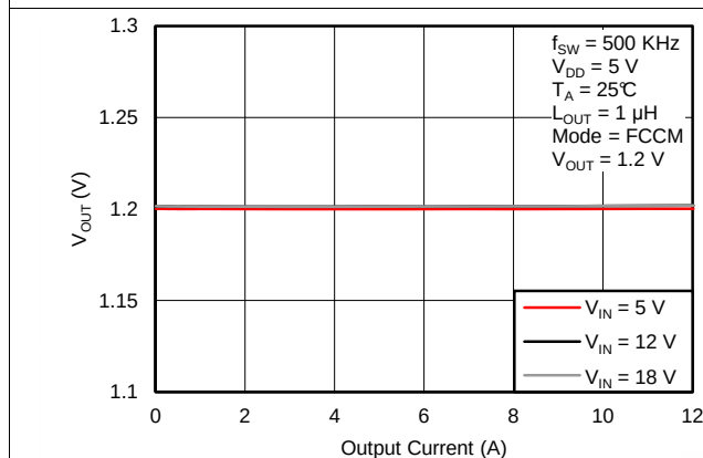
Figure 55. Output Voltage vs. Output Current
