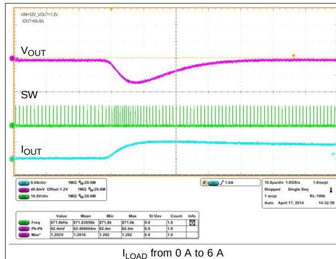
Figure 59. Load Transient
