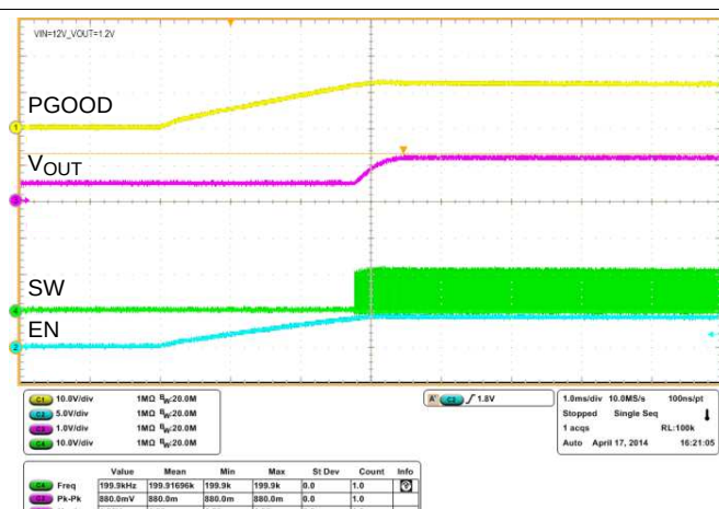
Figure 64. Pre-Bias Start-Up
