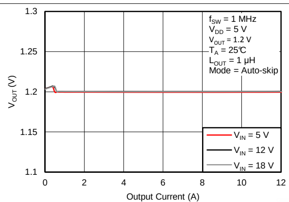
Figure 54. Output Voltage vs. Output Current
