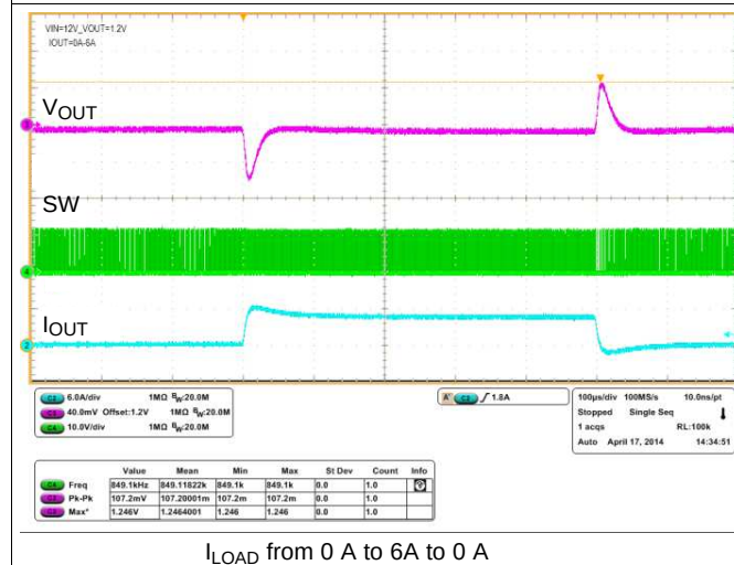
Figure 61. Full Cycle Load Transient
