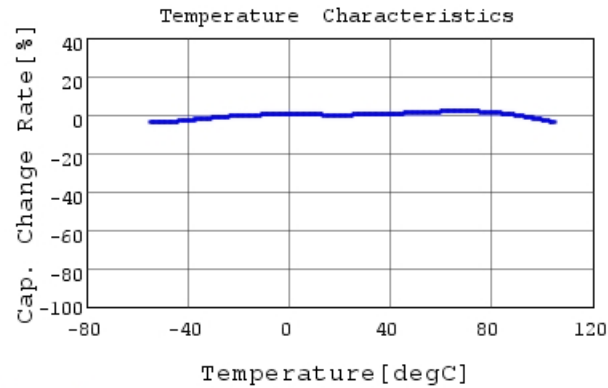
GRM155C8YA224KE01 C-Temp. capchange, DC0.0V,
