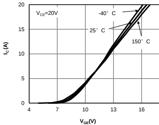
Fig 3: Transfer Characteristic
