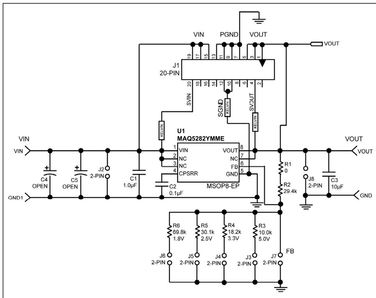
FIGURE 6-1: MAQ5282 Evaluation Board Schematic.
