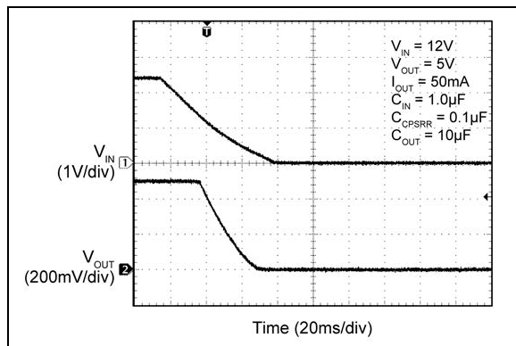
FIGURE 2-20: Soft Turn-Off.
