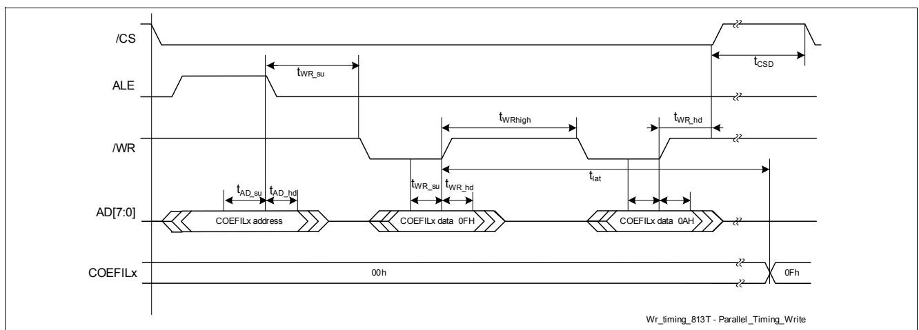
Figure 6 Timing Diagram \mu C Control Mode Write
