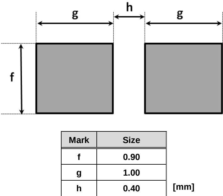
Fig. 3 Land Pattern
