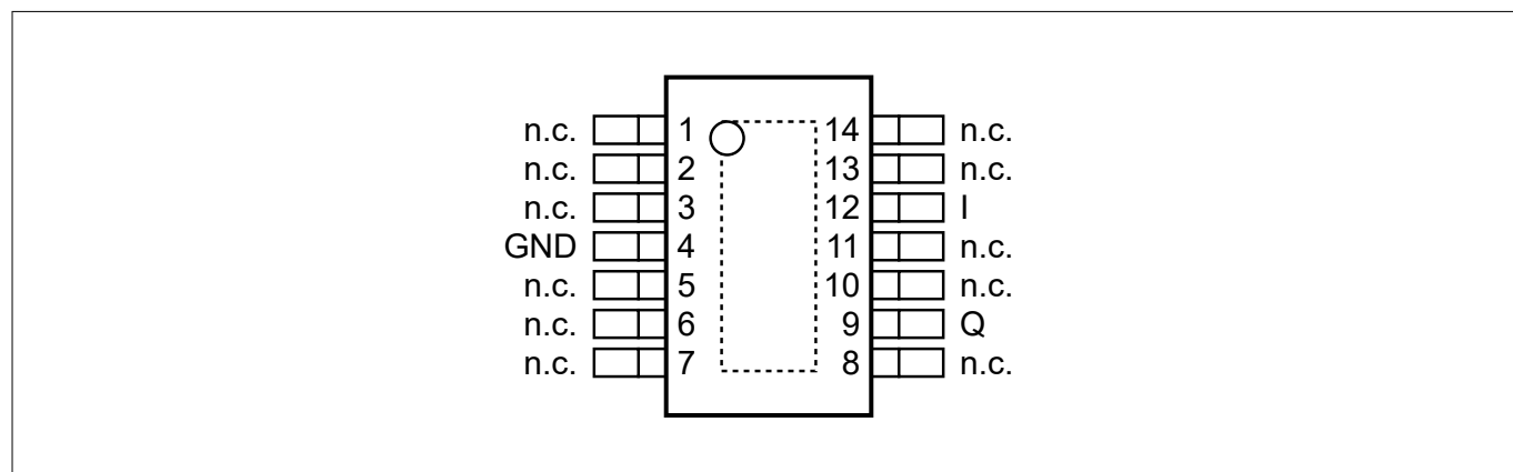
Figure 2 Pin assignment
