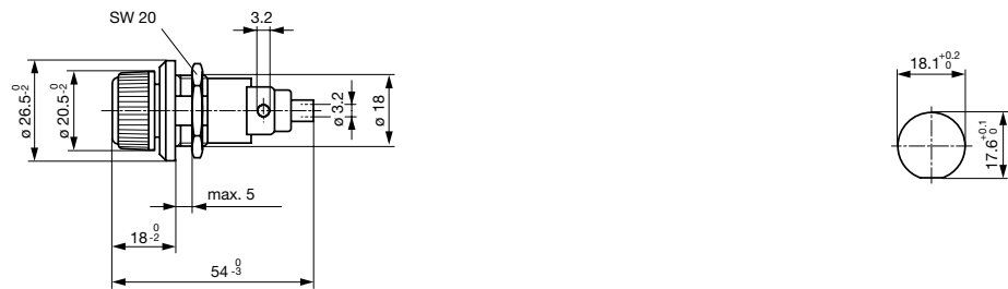
Mounting holes
