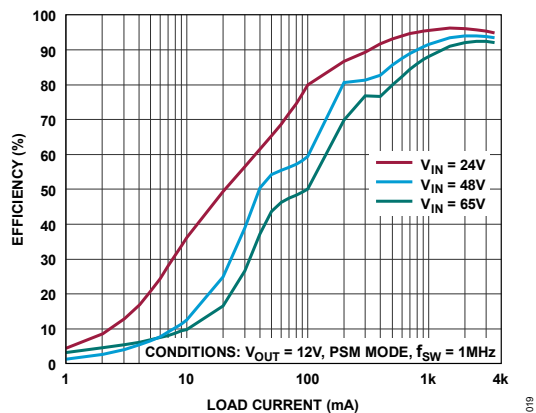
Figure 19. LT80603 Efficiency vs. Load Current
