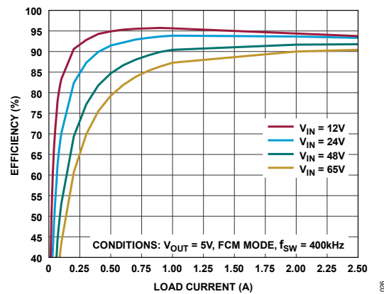
Figure 26. LT80602 Efficiency vs. Load Current
