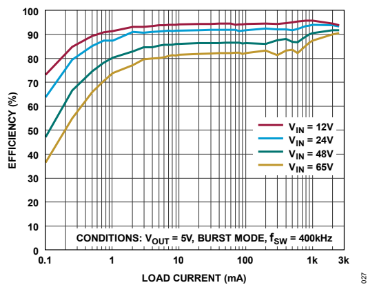
Figure 27. LT80602 Efficiency vs. Load Current
