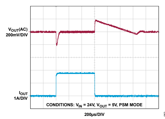
Figure 62. LT80603 Load Current Stepped from 10mA to 1.75A (See Figure 82, Typical Application Circuit)
