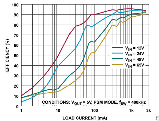
Figure 28. LT80602 Efficiency vs. Load Current
