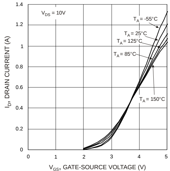
Fig. 10 Transfer Characteristics
