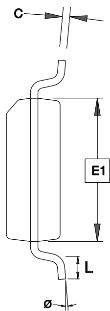
END VIEW
