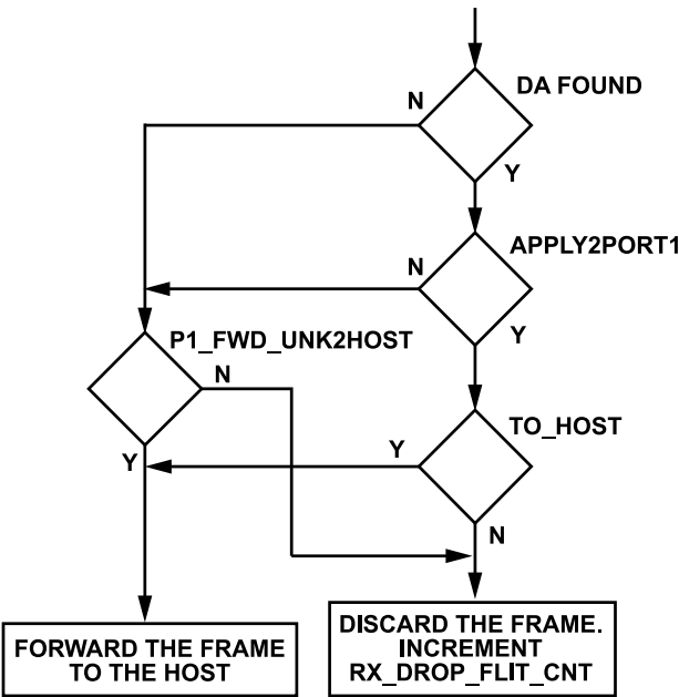
Figure 30. Filtering Algorithm
