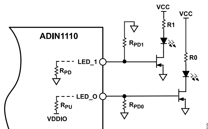
Figure 18. Recommended Transistor Controlled LED Circuit
