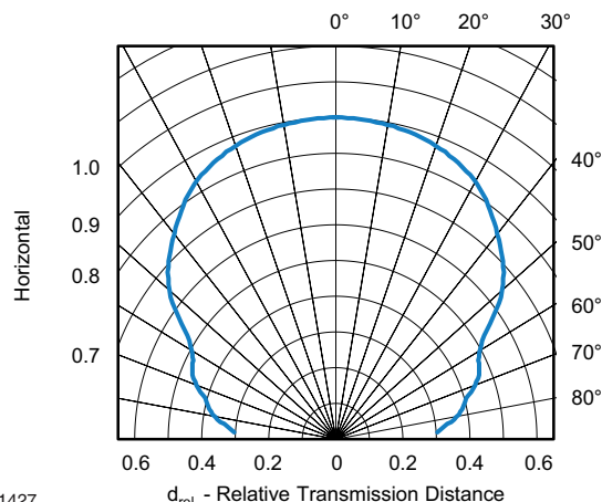
Fig. 3 - Horizontal Directivity
