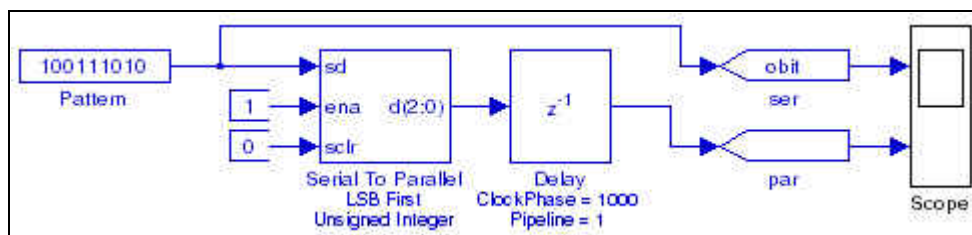
Figure 25–10. Serial To Parallel Block Example
