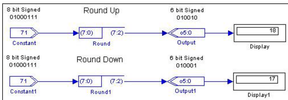
Figure 20-12. Round Block Example
