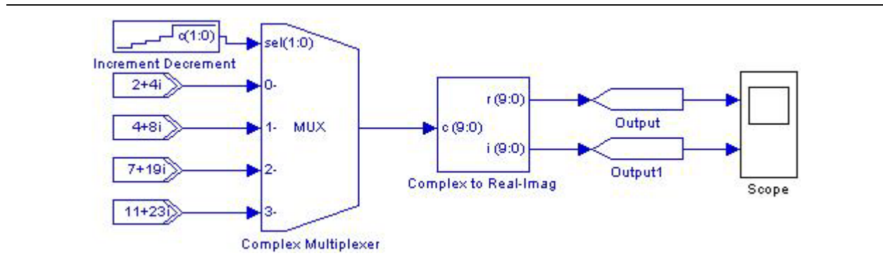
Figure 17-6. Complex Multiplexer Block Example
