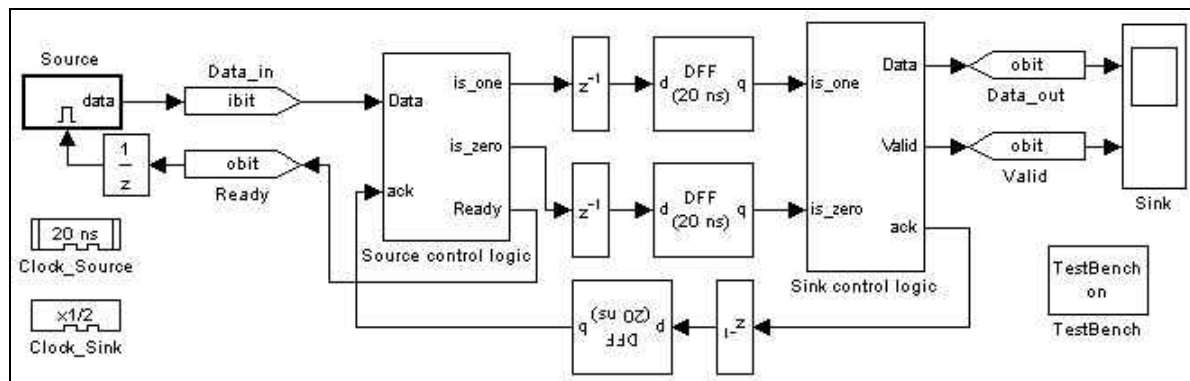
Figure 22-1. Multirate DFF Block Example
