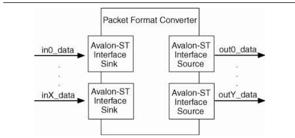
Figure 19-7. Basic Packet Format Converter
