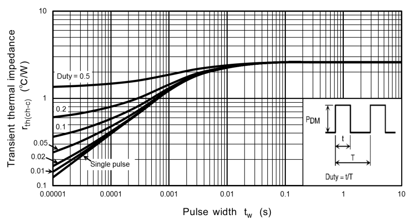
Fig. 8.13 r_{th} - t_w (Guaranteed Maximum)
