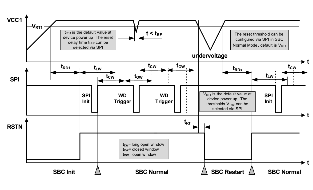
Figure 37 Reset Timing Diagram
