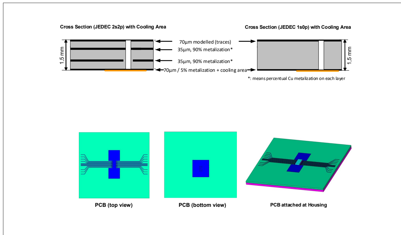
Figure 55 Board Setup
