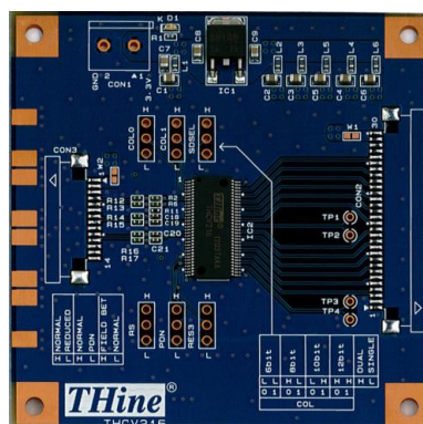
(b) THEVA216-V2 (Top Side)
