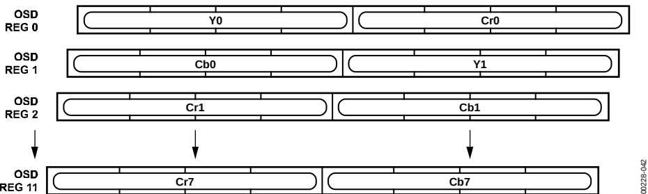
Figure 42. OSD Registers
