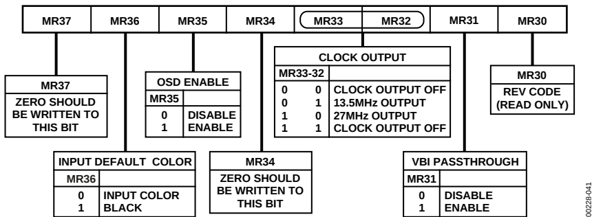
Figure 41. Mode Register 3
