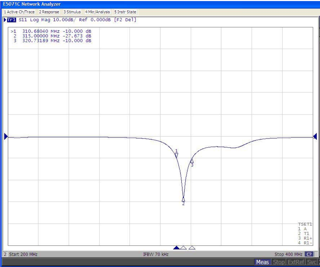
Fig. 4 Return loss
