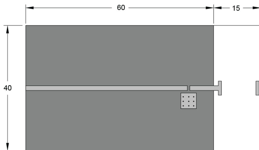
Fig. 2 Outlook and dimension of evaluation board
