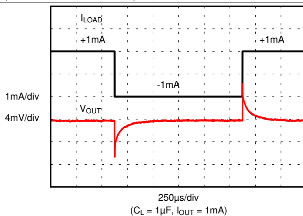
Figure 8. Load Transient
