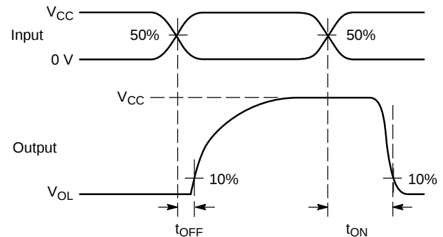
Figure 21. t_{ON}/t_{OFF}
