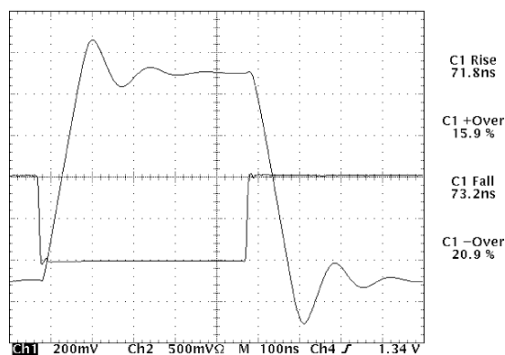
Figure 50. LMV796 Response
