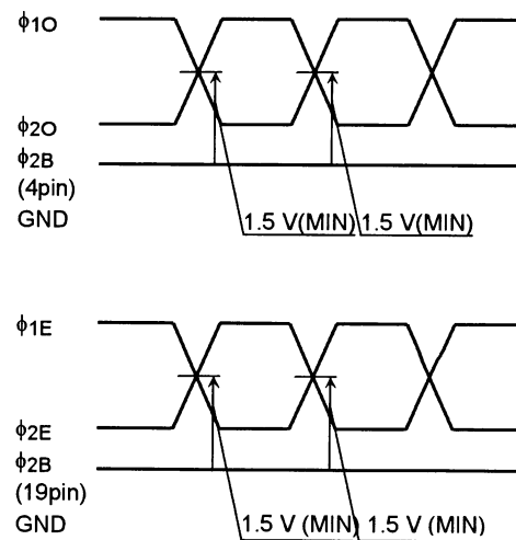
\phi_1 , \phi_2 CROSS POINT
