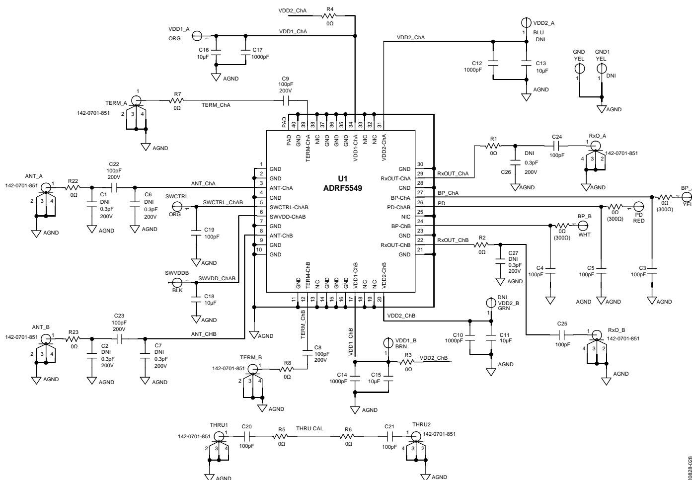
Figure 28. Typical Application Circuit
