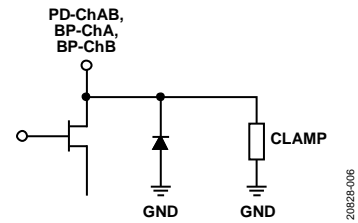
Figure 6. PD-ChAB and BP-Chx Interface Schematic
