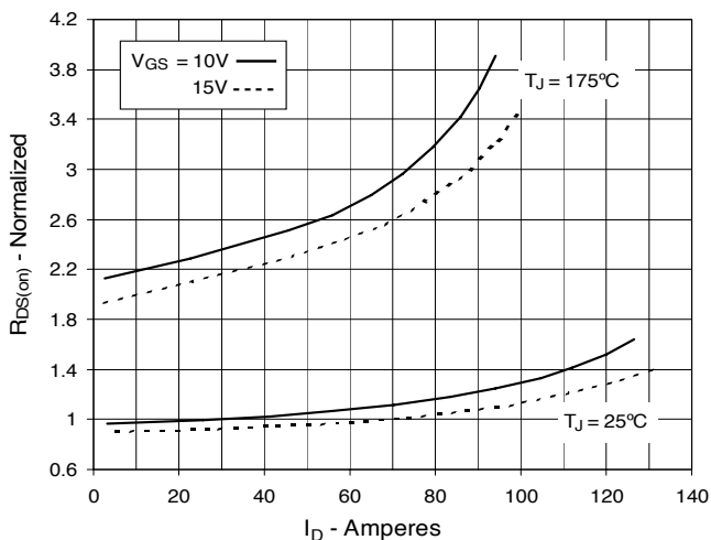
Fig. 5. R_{DS(on)} Normalized to I_D = 27.5A Value vs. Drain Current
