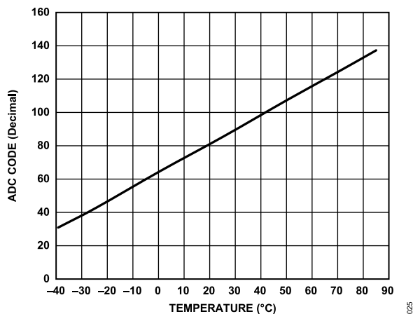
Figure 24. ADC Code vs. Temperature
