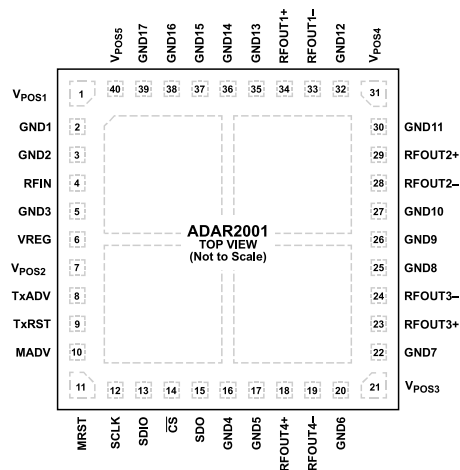
Figure 6. Pin Configuration (Top View, Not to Scale)
