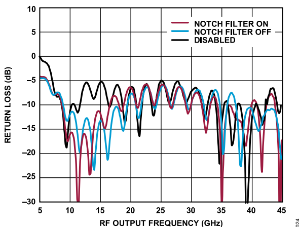
Figure 23. RF Output Return Loss
