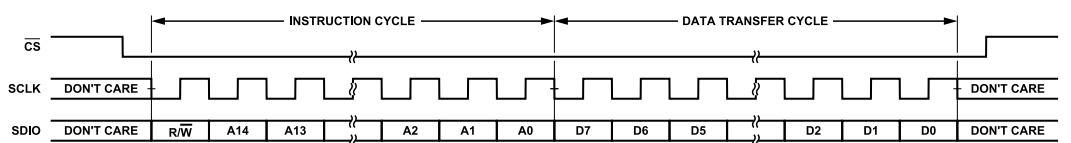
Figure 2. SPI Transaction Structure (MSB First)
