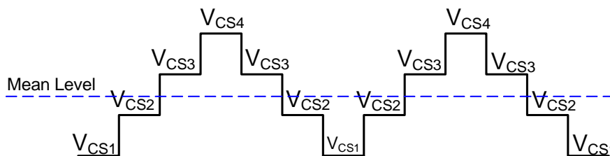
Figure 7: V_{CS} Jitter
